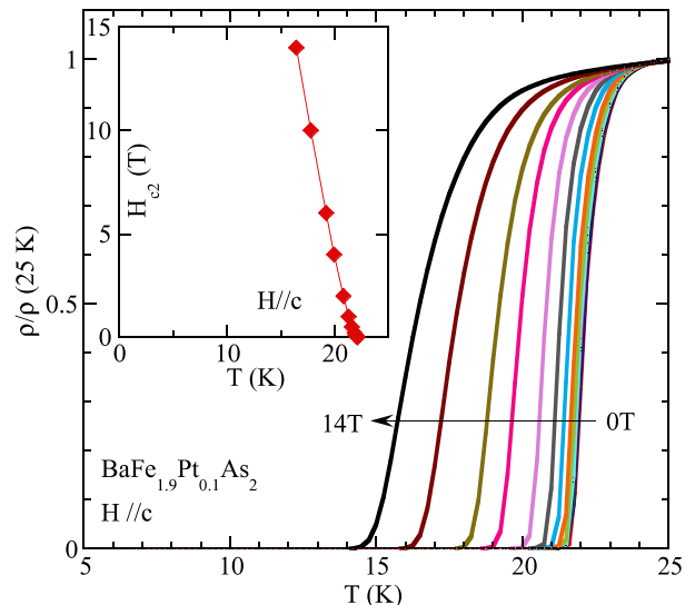
Figure 2. In-plane electrical resistivity of \text{BaFe}_{1.90}\text{Pt}_{0.10}\text{As}_2 in magnetic fields ( 0, 0.01, 0.02, 0.03, 0.04, 0.05, 0.1, 0.2, 0.5, 1, 2, 4, 6, 10 and 14 T indicated by the direction of the arrow) applied along the c -axis, showing the suppression of the superconducting transition by increasing field. The resistivity is normalized to the normal-state value (at 25 K) just above the transition for clarity. The inset shows the upper critical field H_{c2} of \text{BaFe}_{1.90}\text{Pt}_{0.10}\text{As}_2 , for H \parallel c , versus temperature. The points here denote the 50% positions of the resistive transitions for each field from the main figure.
